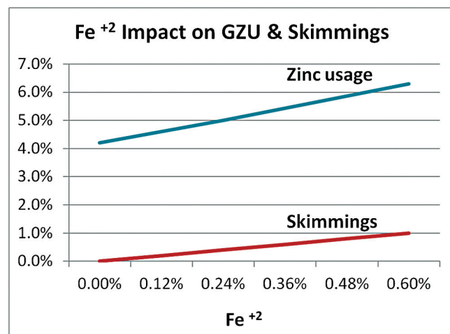
Fig. 1 — Impact of iron contamination in flux tanks.
