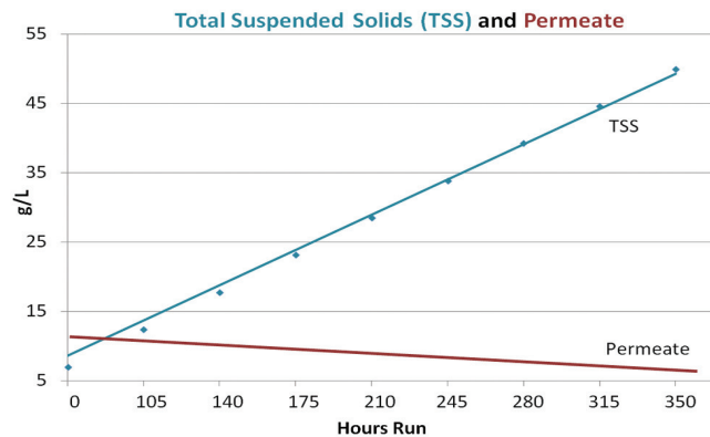
Fig. 9 — Total suspended solids and permeate passing through membrane (Velocity = 10 fps).
