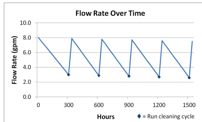
Fig. 10 — Effect of cleaning cycle on flow.
