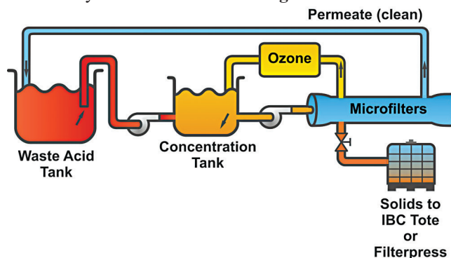
Fig. 4 — Flow diagram - OxyFilter.
