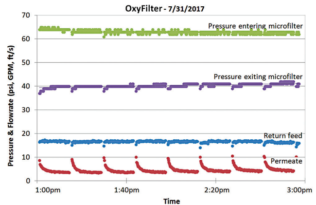
Fig. 8 — Data from the OxyFilter system during the second month of the trial (Pump set to 50+ Hz).
