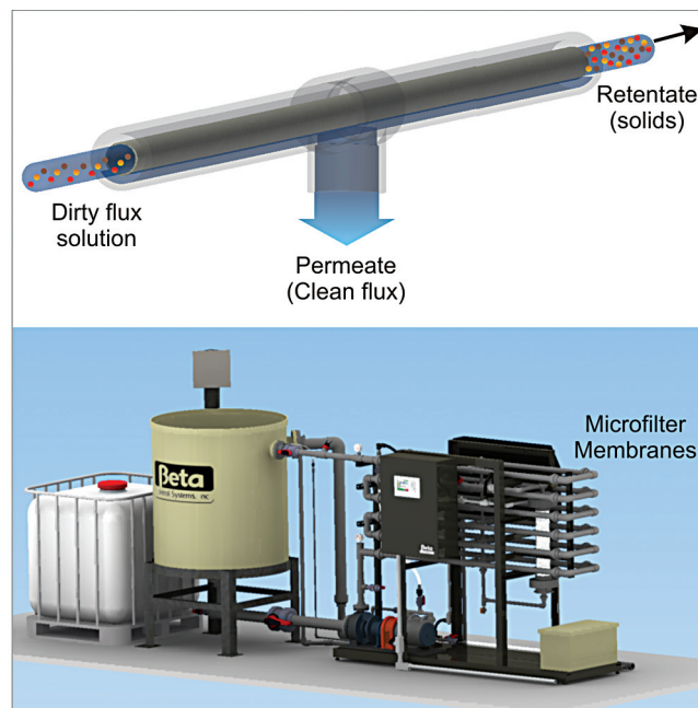
Fig. 2 — OxyFilter using crossflow microfiltration membranes.
